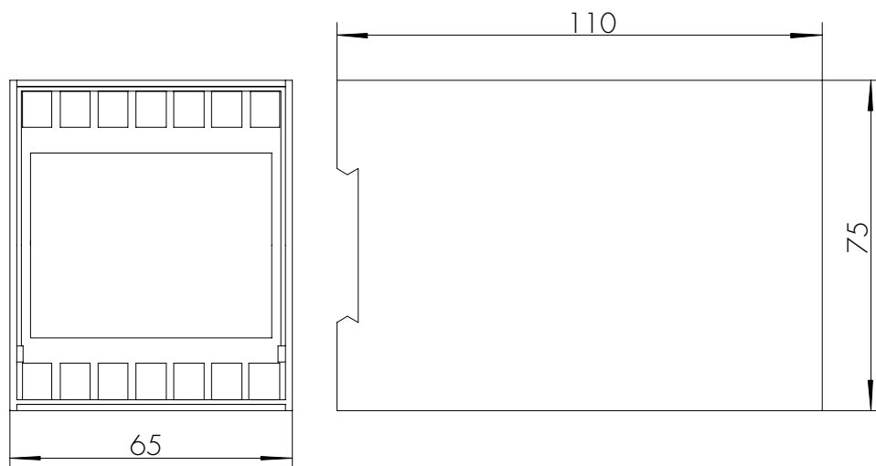
Fig. 5.1: Dimensional drawings
