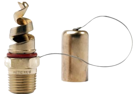
Nozzle with optional protective cover Use of blow-off covers requires a pressure of 25 PSI or higher
