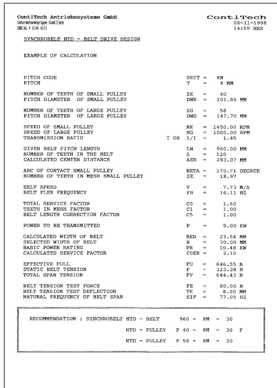
Computer printout for synchronous belt drive design.
