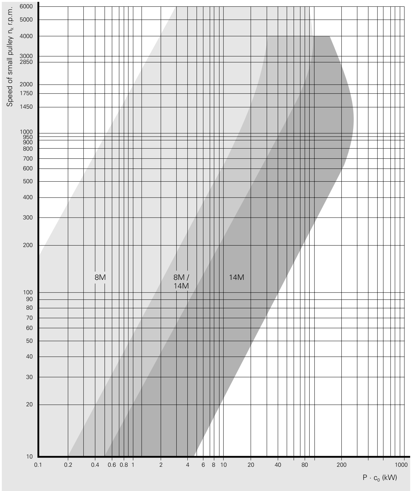
CONTI SYNCHROBELT® HTD Synchronous Drive Belt 8M, 14M
