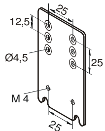
Extension bracket 0 714 146 (incl. screws)
