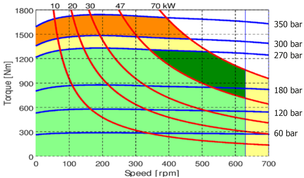
R8M 400 H3
