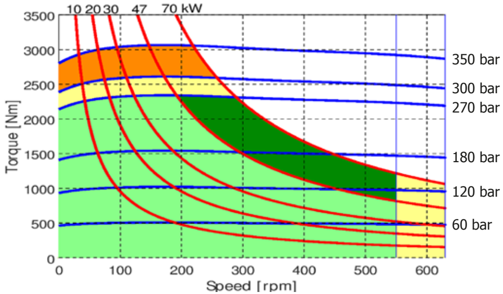
R8M 650 H3
