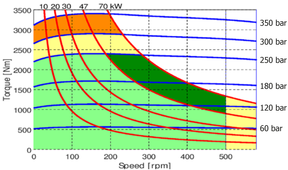
R8M 650 H3
