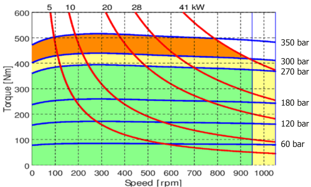
R8M 100 H1
