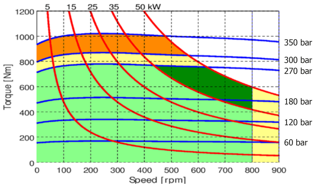
R8M 190 H2
