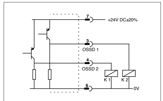
fig 25/3 outputs 1 and 2
