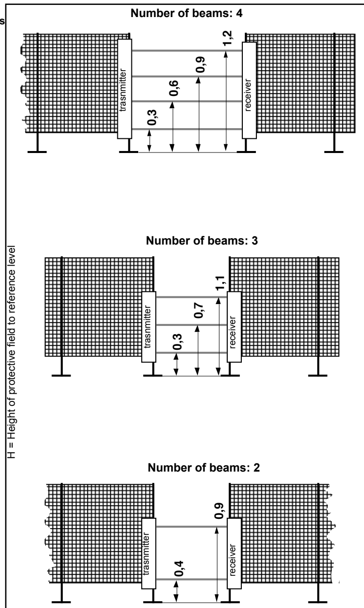
fig 16/1 Vertical protection
