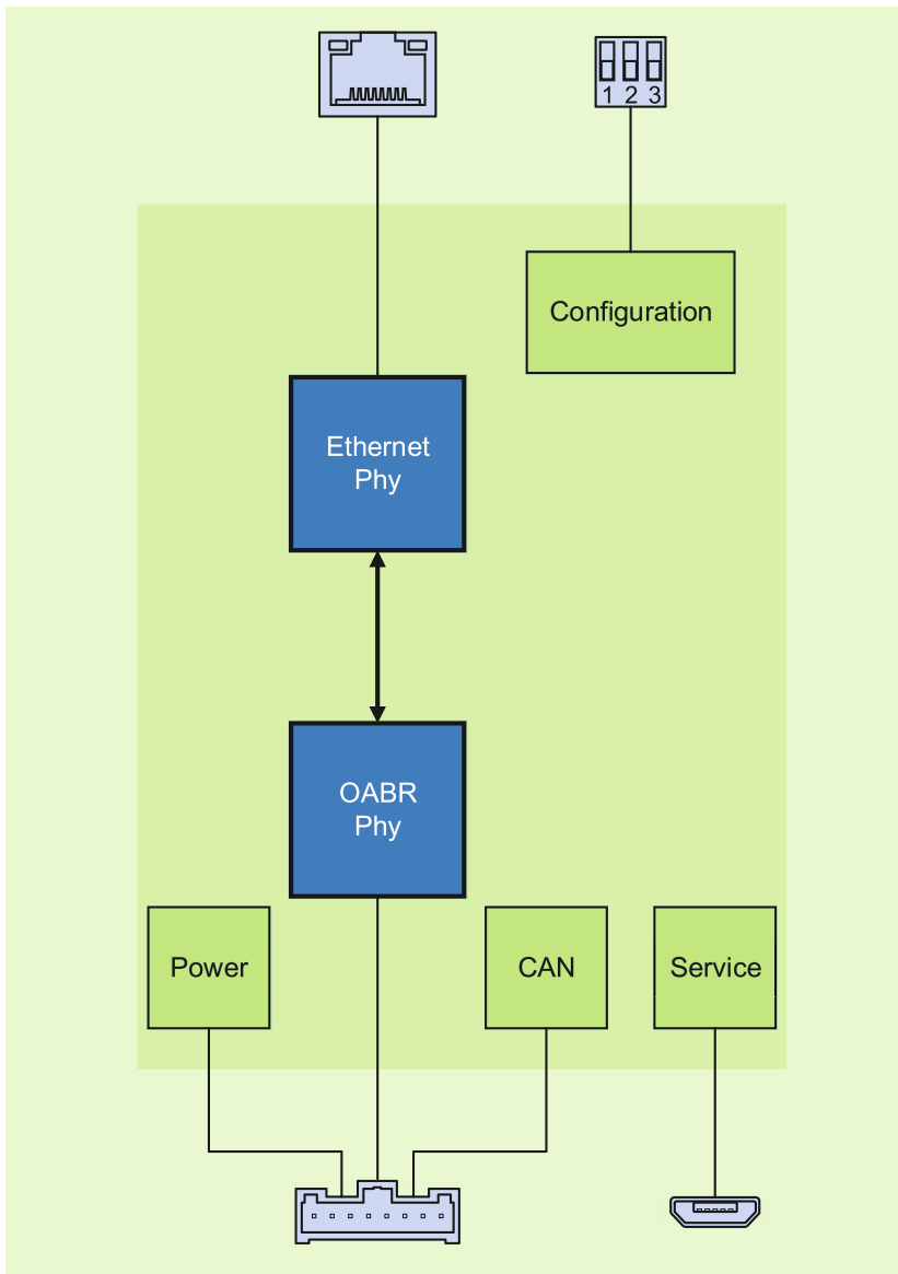
Block diagram
