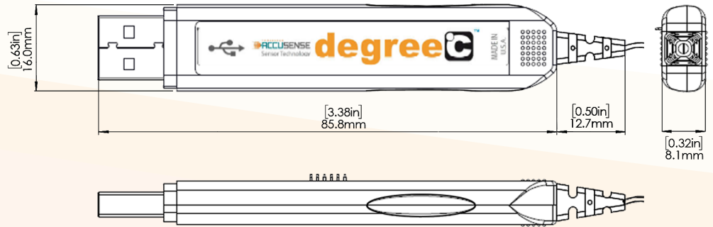
Standard cable length is 5m (16.4') from sensor to connector. Nominal cable diameter is 1.9mm (0.1").
