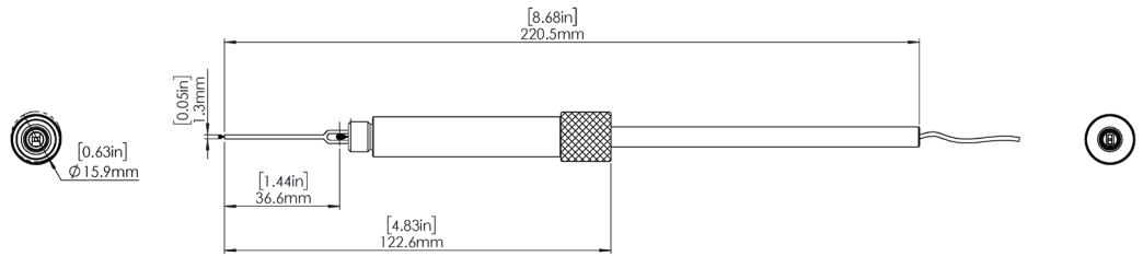
UAS1000 Omnidirectional (OD) Sensor Probe Ideal for high circuit densities and concentrated component arrangements. Contact Degree Controls for a 3D STEP file of the UAS1000 OD sensor probe.
