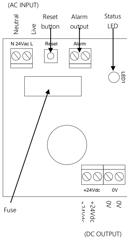
PS-24-24DC-1A:
