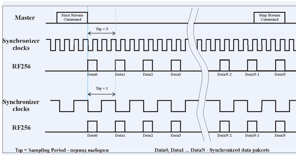
Data stream transfer with external synchronization
