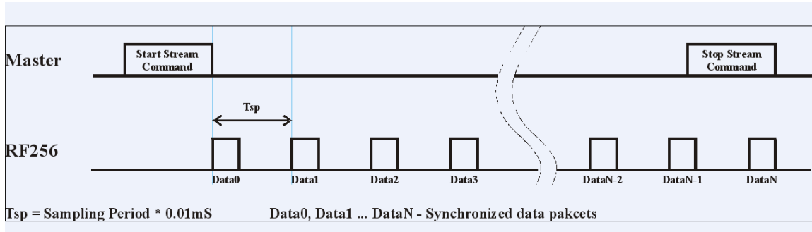
Data stream transfer with time synchronization
