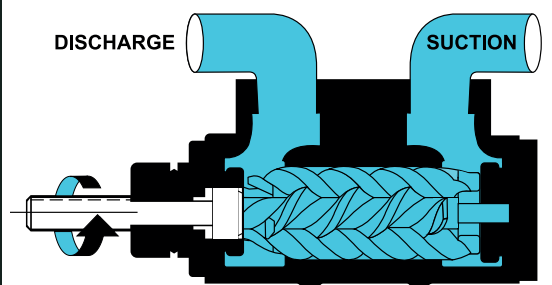
TRIRO FLOW PRINCIPLE
