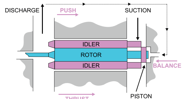
HYDRAULIC BALANCE
