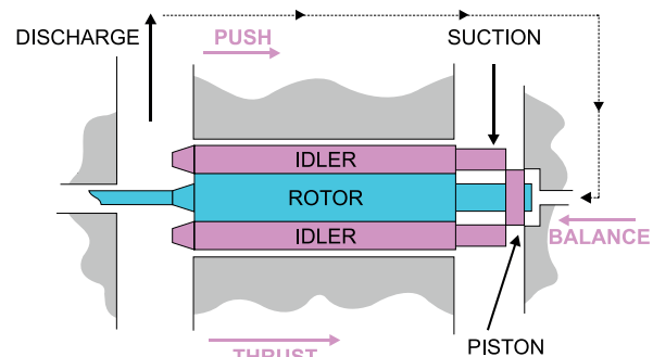
TRIRO FLOW PRINCIPLE
